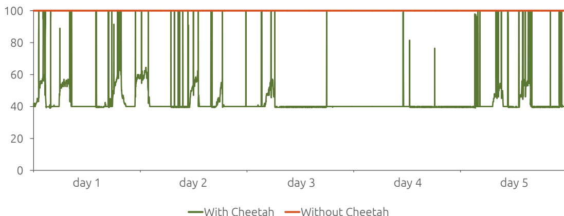
Park Inn Lille: engine RPM with and without Cheetah (in %)
